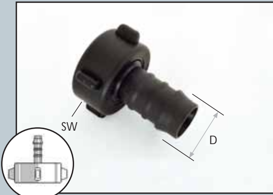
Polypropylene swivel hose connector with flat seal. Good resistance to chemicals and fertilizers. Suitable for outdoors use in irrigation systems and gardens.
